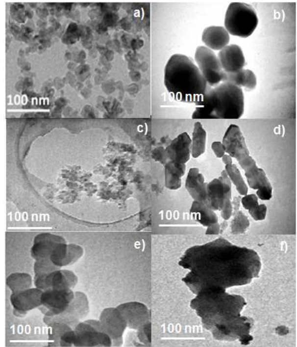
Figure 6. TEM images of (a) SiC, (b) PPy, (c) Fc/SiC, (d) Fc-PPy, (e) Fc/SiC & (f) Fc-PPy/SiC low sample.
