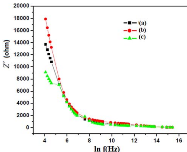
Figure 7. Real impedance ( Z' ) versus \ln(f) for a) \text{LaMnO}_3 b) \text{La}_{0.8}\text{Sr}_{0.1}\text{Co}_{0.1}\text{MnO}_3 c) \text{La}_{0.8}\text{Sr}_{0.1}\text{Fe}_{0.1}\text{MnO}_3 of cathode materials.
