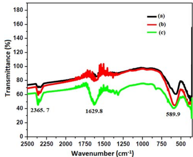
Figure 5. FT-IR spectra of a) LaMnO 3 b) La 0.8 Sr 0.1 Co 0.1 MnO. c) La 0.8 Sr 0.1 Fe 0.1 MnO 3 of cathode materials.
