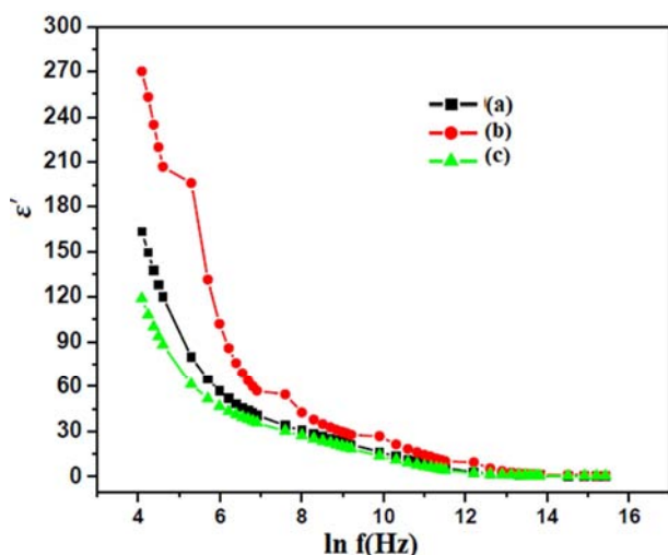
Figure 9. The variation of dielectric constant \epsilon' with frequency for a) LaMnO 3 b) La 0.8 Sr 0.1 Co 0.1 MnO 3-δ c) La 0.8 Sr 0.1 Fe 0.1 MnO 3-δ of cathode materials.
